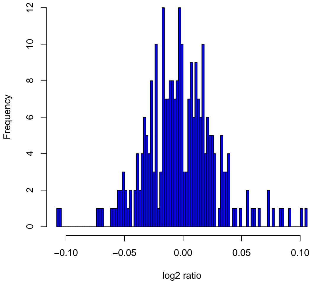
Histogram of log2ratios in 270 HapMap samples at clone Chr6tp-3G2
