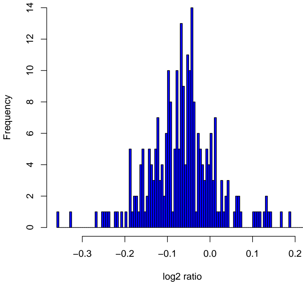
Histogram of log 2 ratios in 270 HapMap samples at clone Chr6tp-4B8
