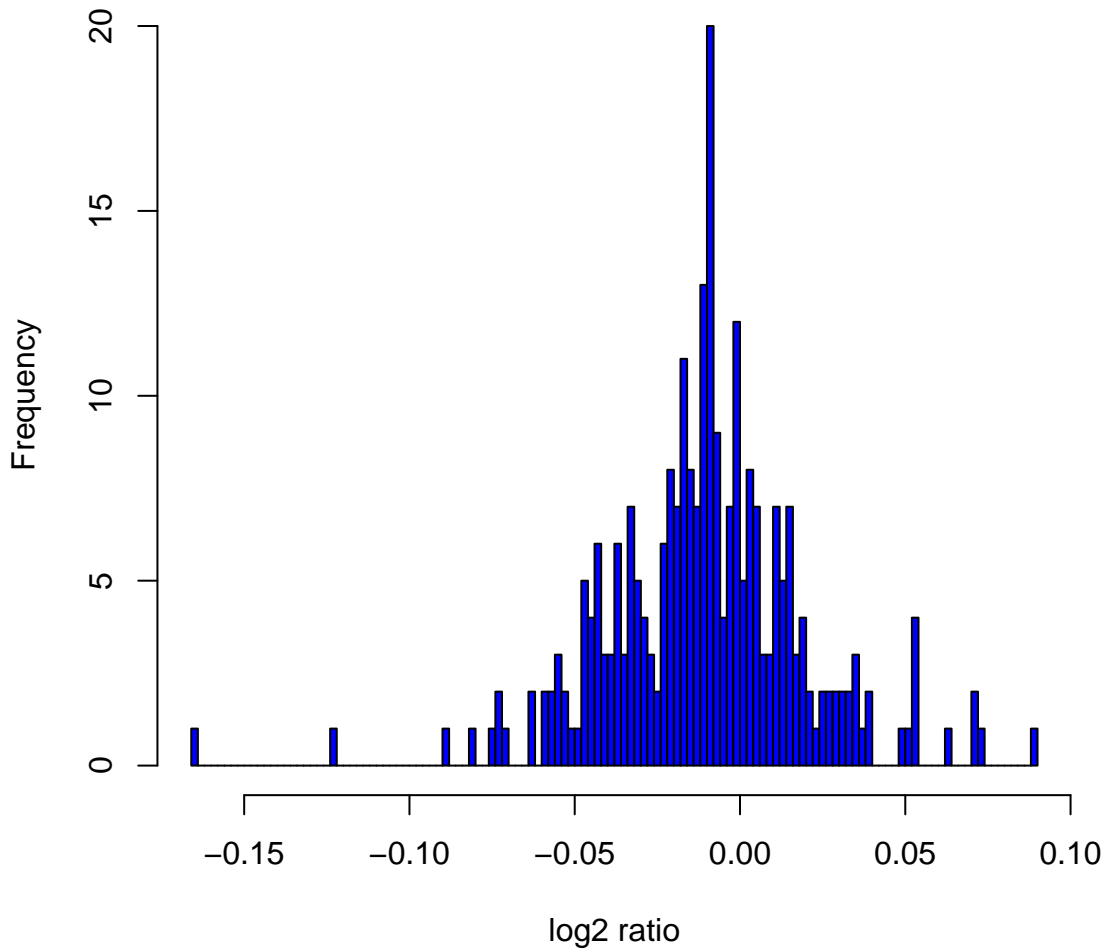
Histogram of log2ratios in 270 HapMap samples at clone Chr6tp-4C12
