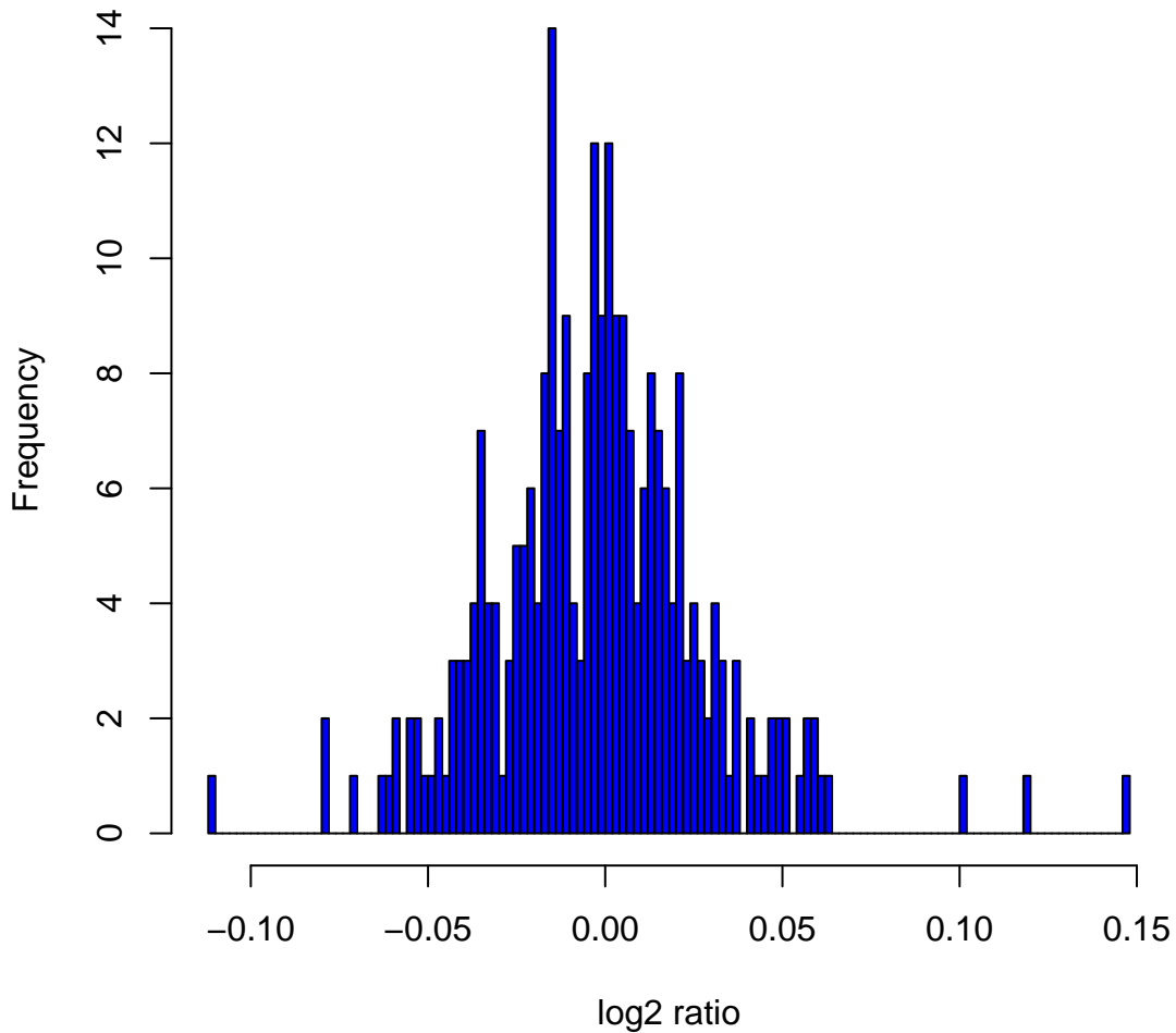
Histogram of log 2 ratios in 270 HapMap samples at clone Chr6tp-4C2
