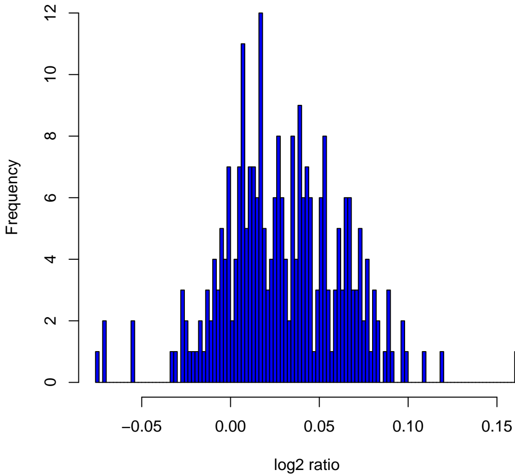
Histogram of \log_2 ratios in 270 HapMap samples at clone Chr6tp-4C5
