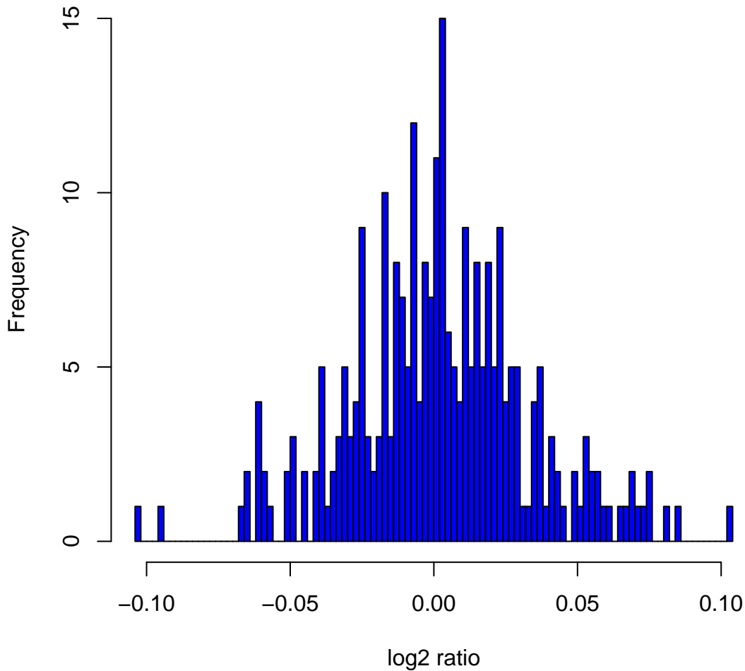
Histogram of log 2 ratios in 270 HapMap samples at clone Chr6tp-4D3
