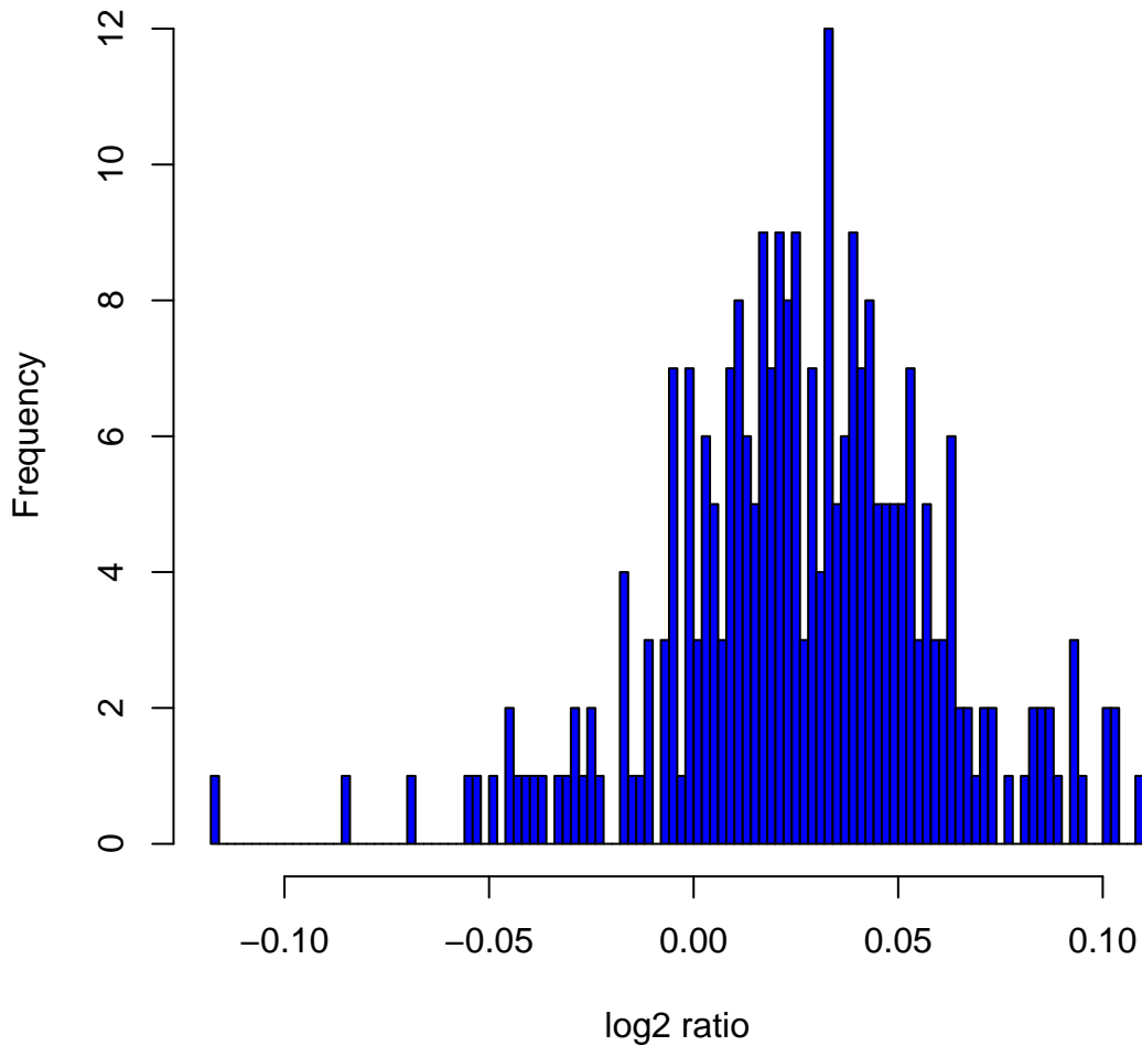
Histogram of log 2 ratios in 270 HapMap samples at clone Chr6tp-4D5
