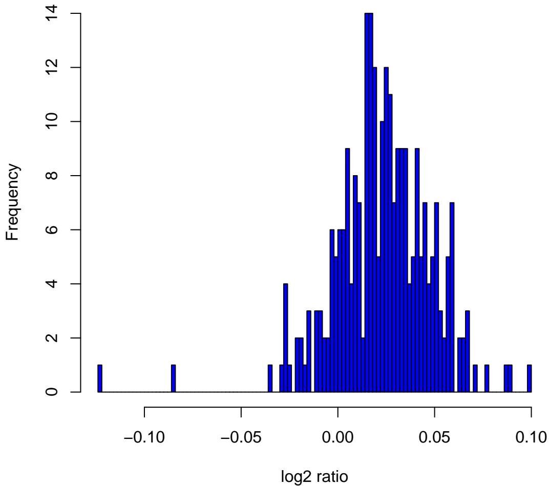
Histogram of log 2 ratios in 270 HapMap samples at clone Chr6tp-4D6
