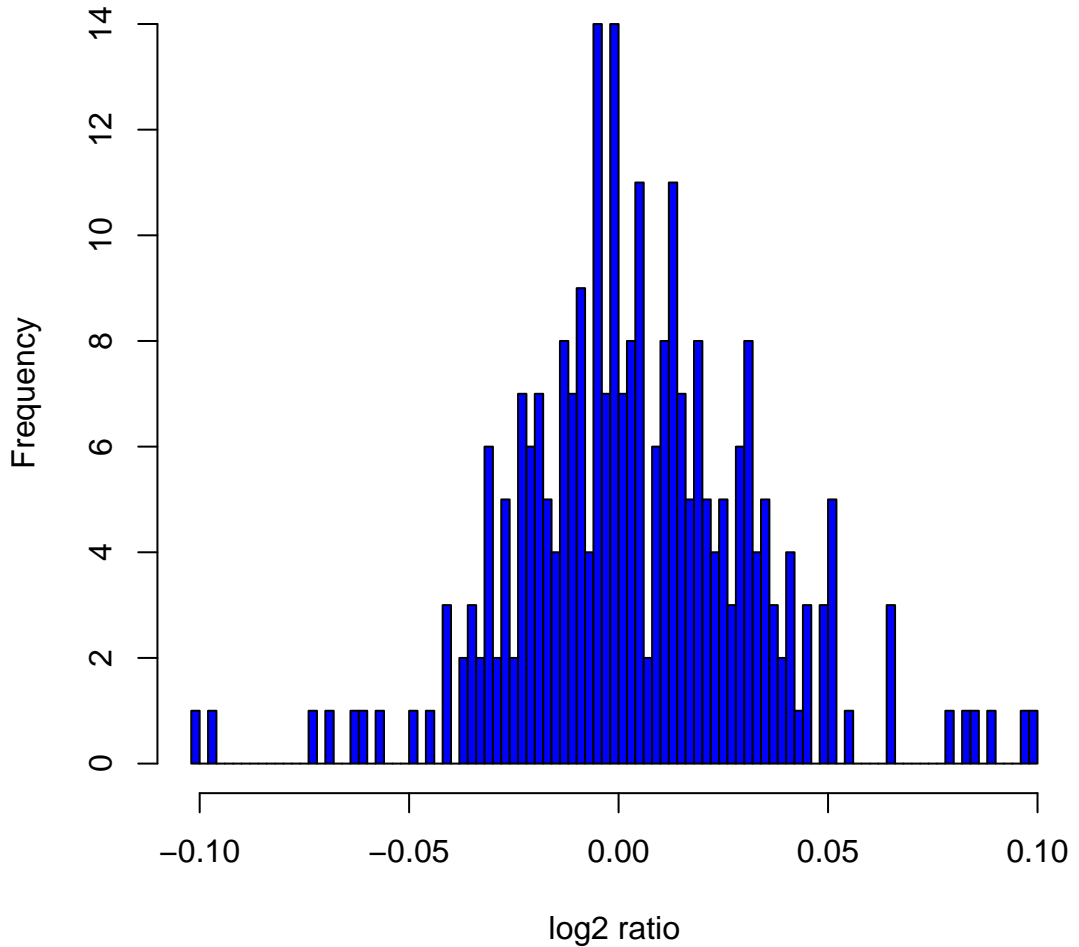
Histogram of log2ratios in 270 HapMap samples at clone Chr6tp-4F9
