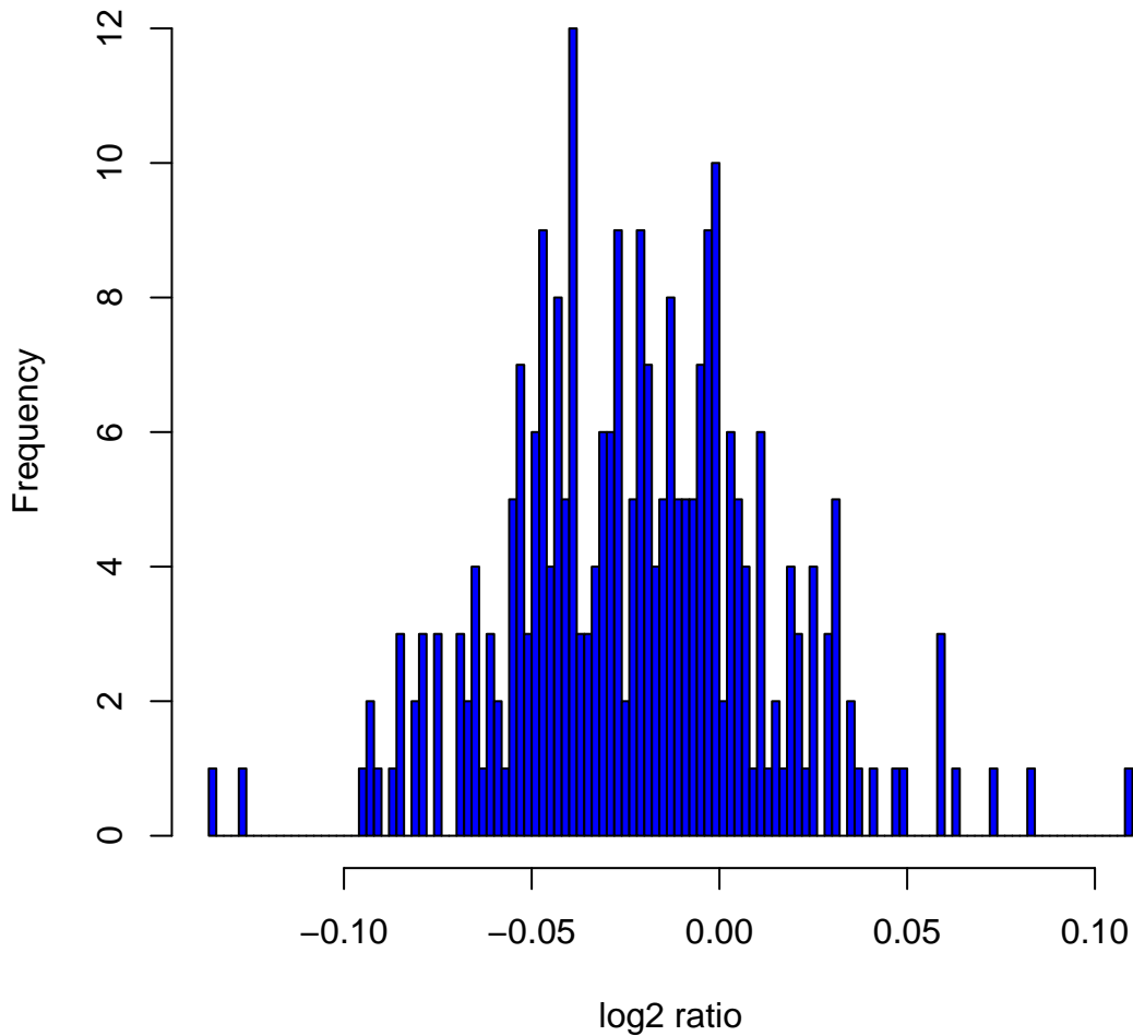
Histogram of \log_2 ratios in 270 HapMap samples at clone Chr6tp-4H9
