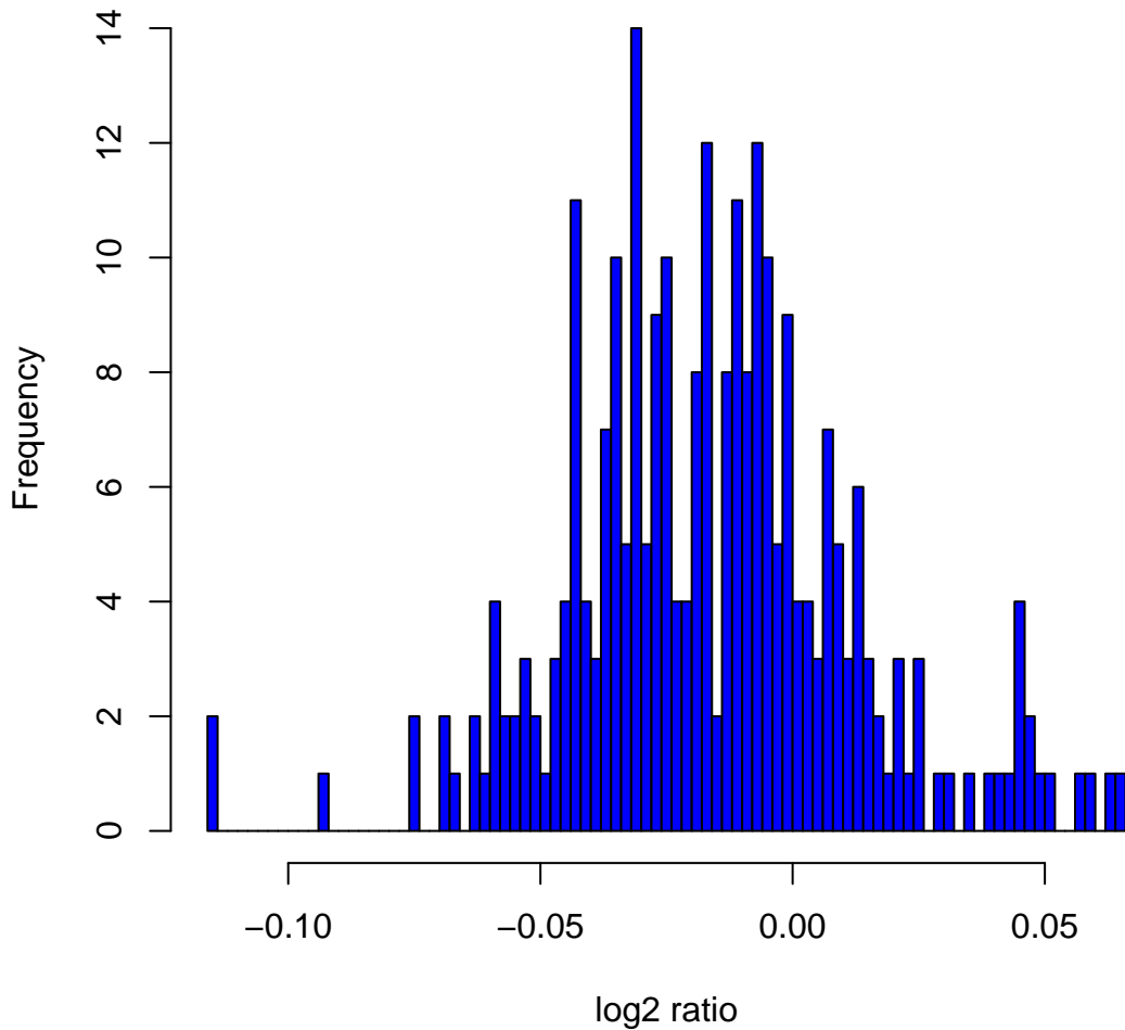
Histogram of \log_2 ratios in 270 HapMap samples at clone Chr6tp-5A2
