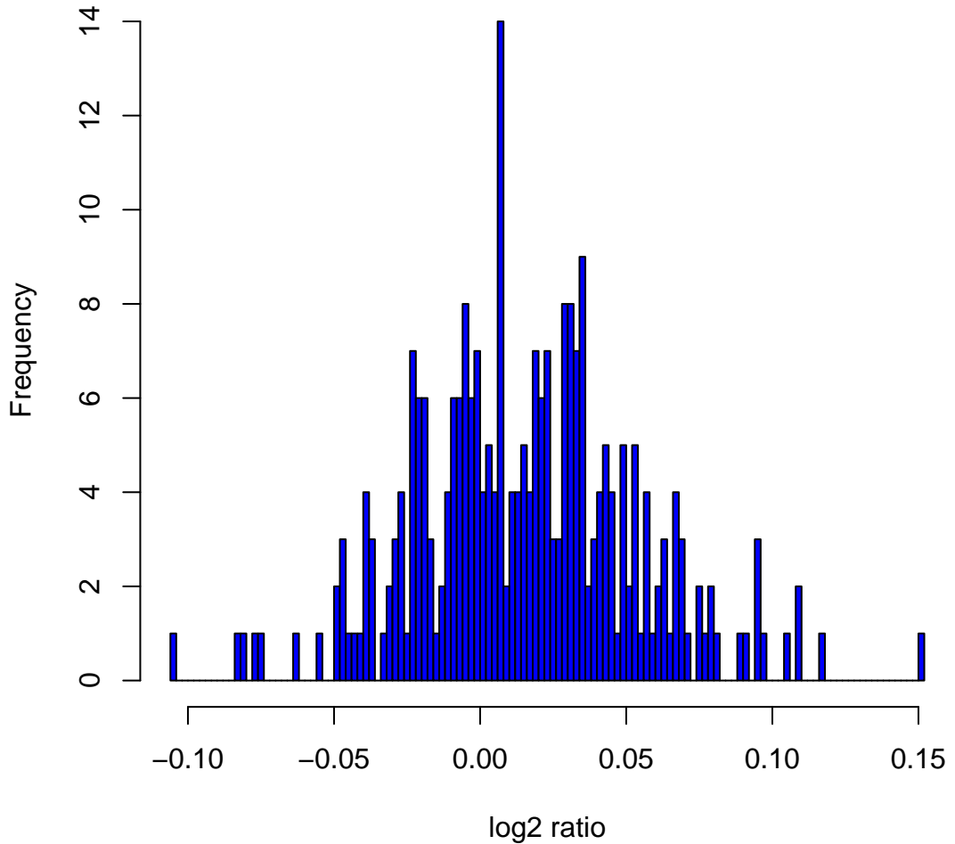
Histogram of log 2 ratios in 270 HapMap samples at clone Chr6tp-5B12
