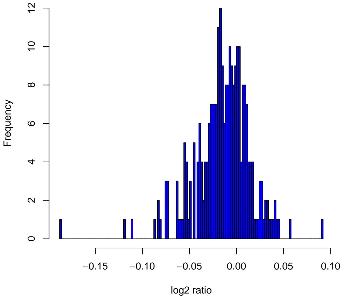
Histogram of log 2 ratios in 270 HapMap samples at clone Chr6tp-5B6
