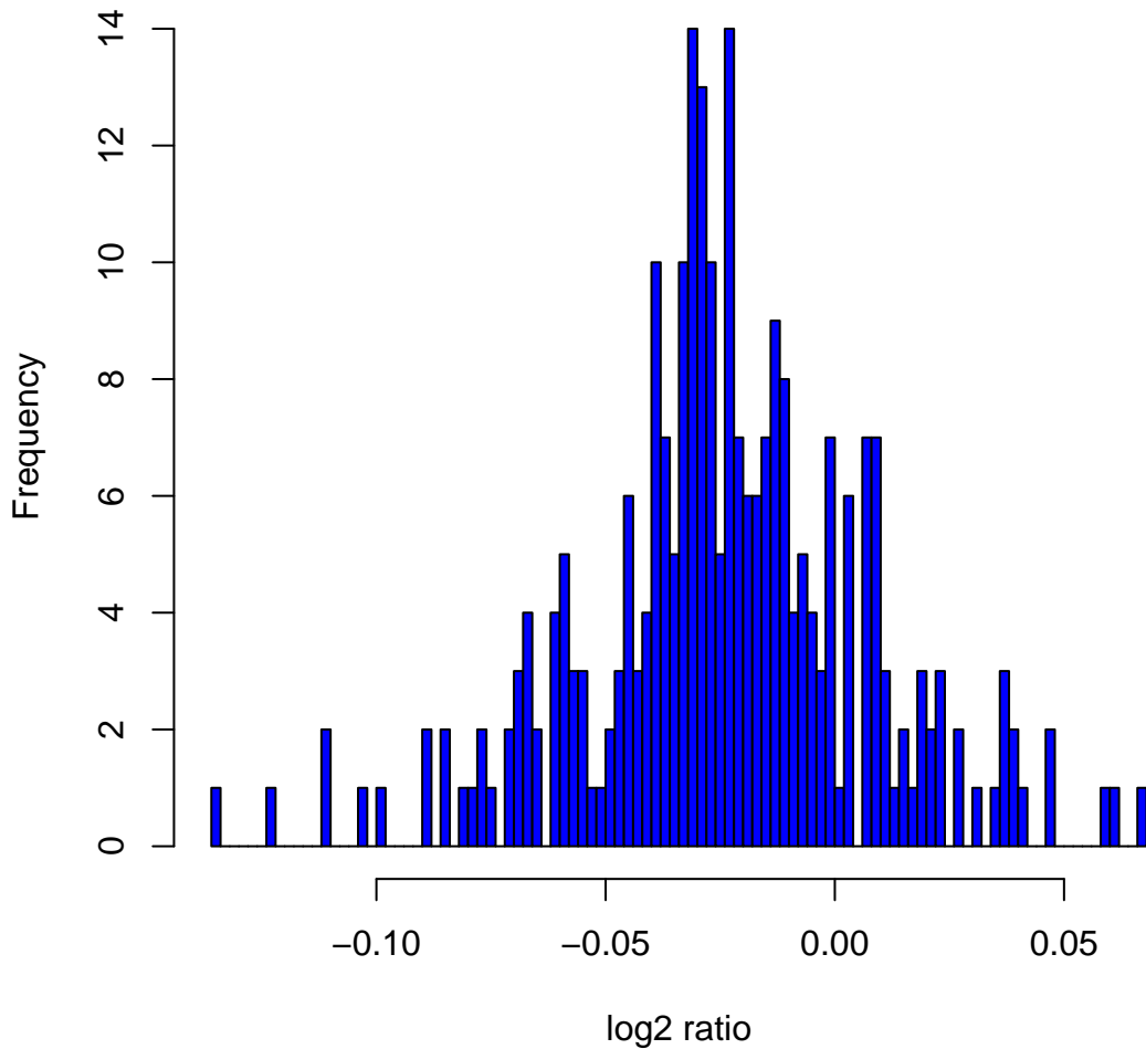
Histogram of log 2 ratios in 270 HapMap samples at clone Chr6tp-5D11
