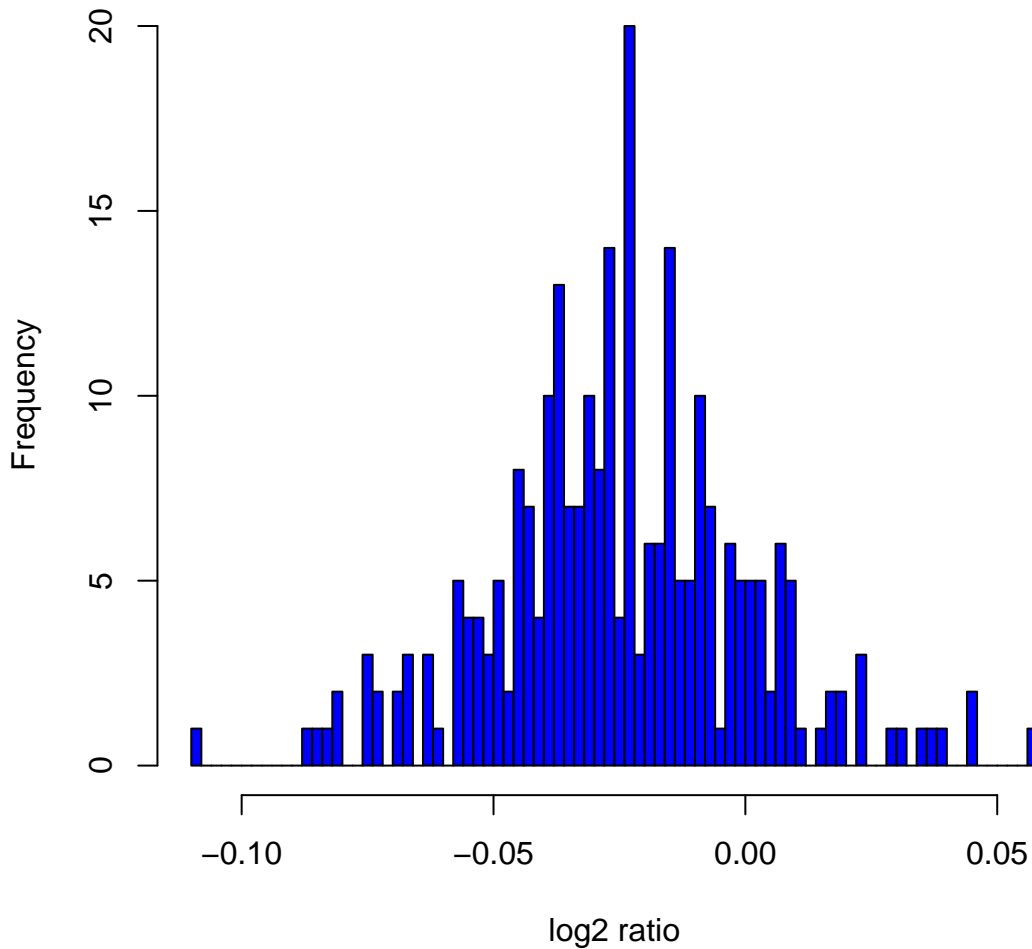
Histogram of log 2 ratios in 270 HapMap samples at clone Chr6tp-5D5
