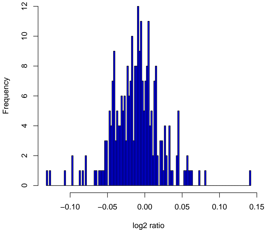
Histogram of log 2 ratios in 270 HapMap samples at clone Chr6tp-5D7
