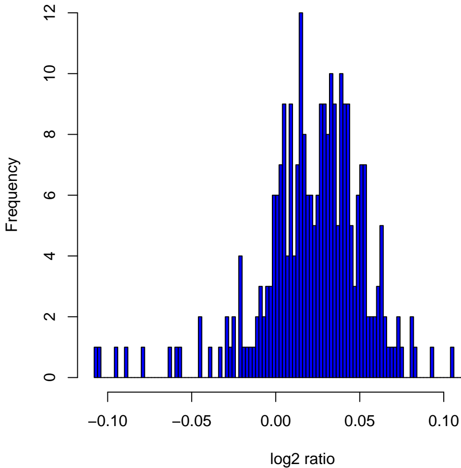
Histogram of log 2 ratios in 270 HapMap samples at clone Chr6tp-5E9
