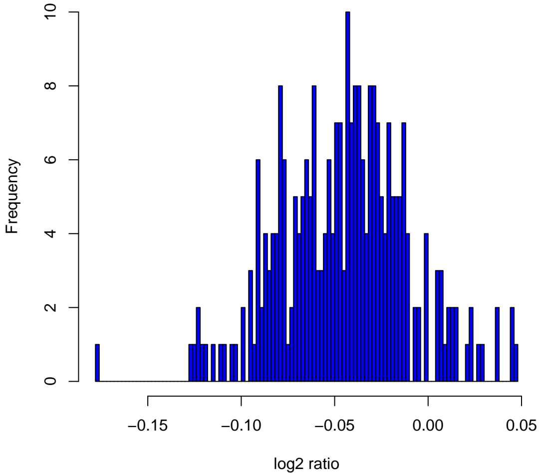
Histogram of log2ratios in 270 HapMap samples at clone Chr6tp-5F4
