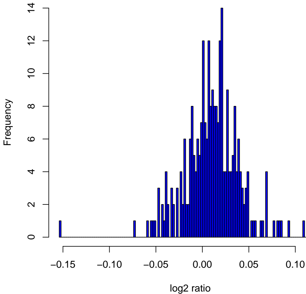
Histogram of log 2 ratios in 270 HapMap samples at clone Chr6tp-6B11
