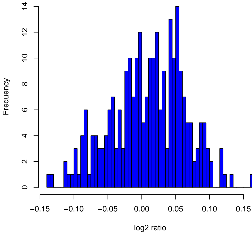
Histogram of log 2 ratios in 270 HapMap samples at clone Chr6tp-6B2
