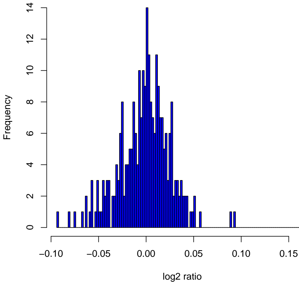
Histogram of log 2 ratios in 270 HapMap samples at clone Chr6tp-6B8
