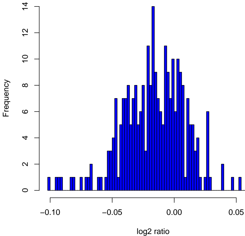
Histogram of \log_2 ratios in 270 HapMap samples at clone Chr6tp-6C3
