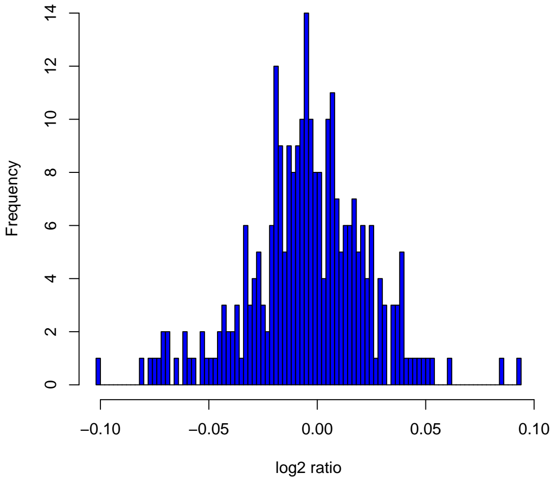
Histogram of log2ratios in 270 HapMap samples at clone Chr6tp-6C5
