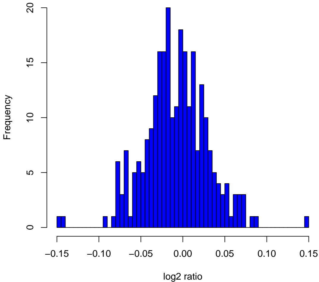
Histogram of log 2 ratios in 270 HapMap samples at clone Chr6tp-6C6
