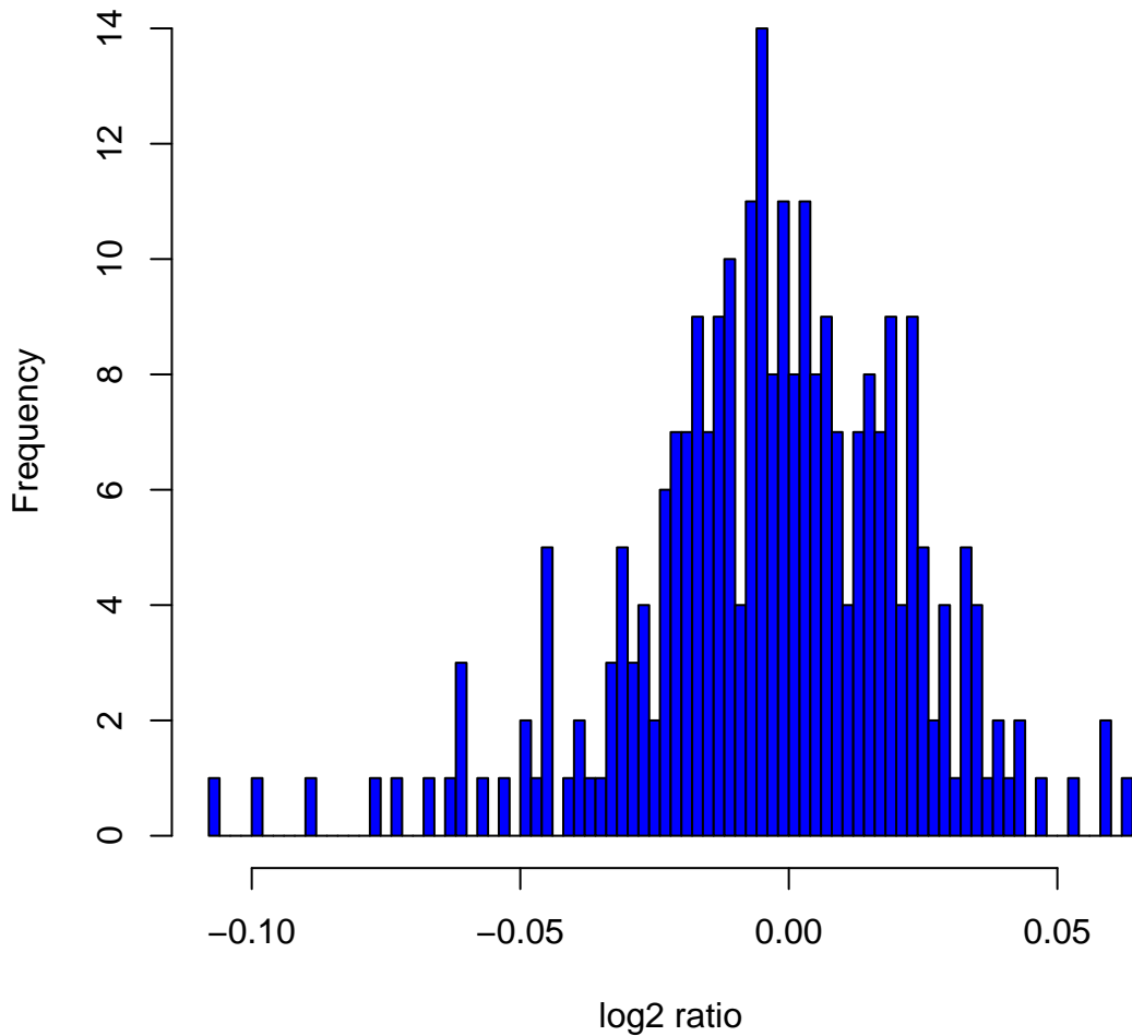
Histogram of \log_2 ratios in 270 HapMap samples at clone Chr6tp-6D4
