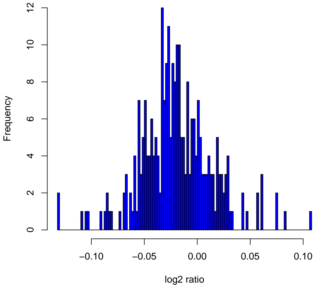
Histogram of \log_2 ratios in 270 HapMap samples at clone Chr6tp-6D8
