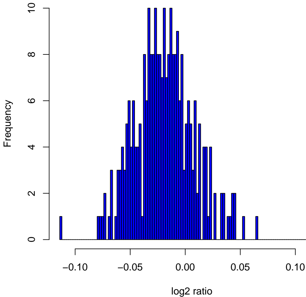
Histogram of \log_2 ratios in 270 HapMap samples at clone Chr6tp-6G1
