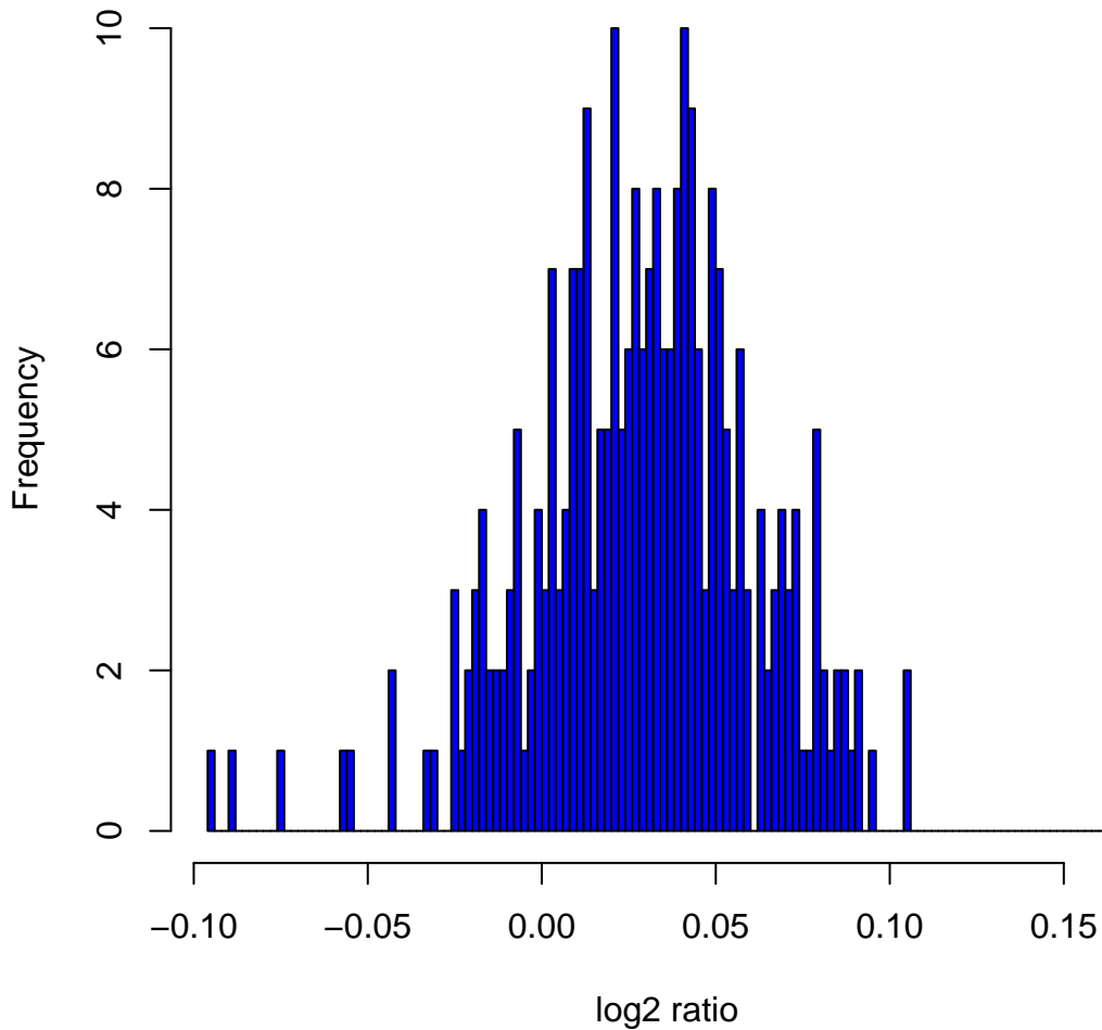
Histogram of log 2 ratios in 270 HapMap samples at clone Chr6tp-6G7
