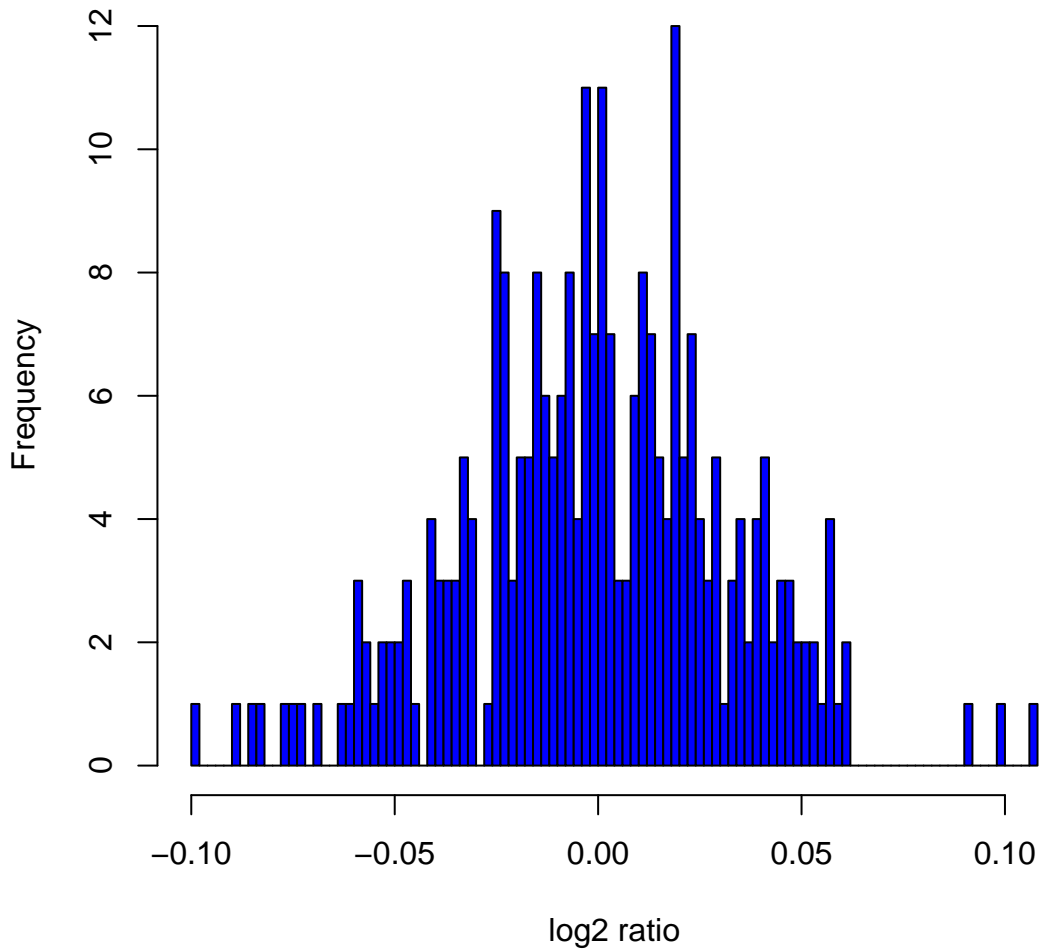
Histogram of log 2 ratios in 270 HapMap samples at clone Chr6tp-6G8
