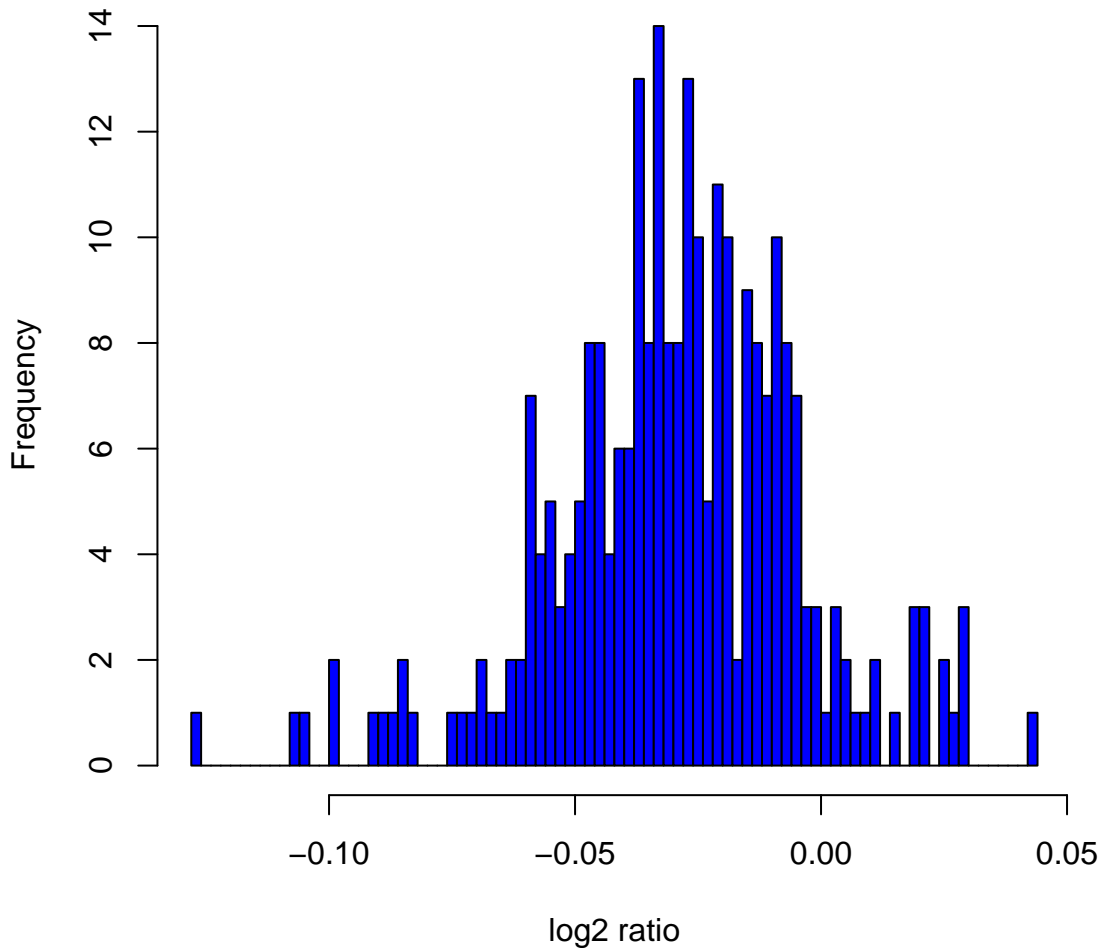
Histogram of log 2 ratios in 270 HapMap samples at clone Chr6tp-6H1
