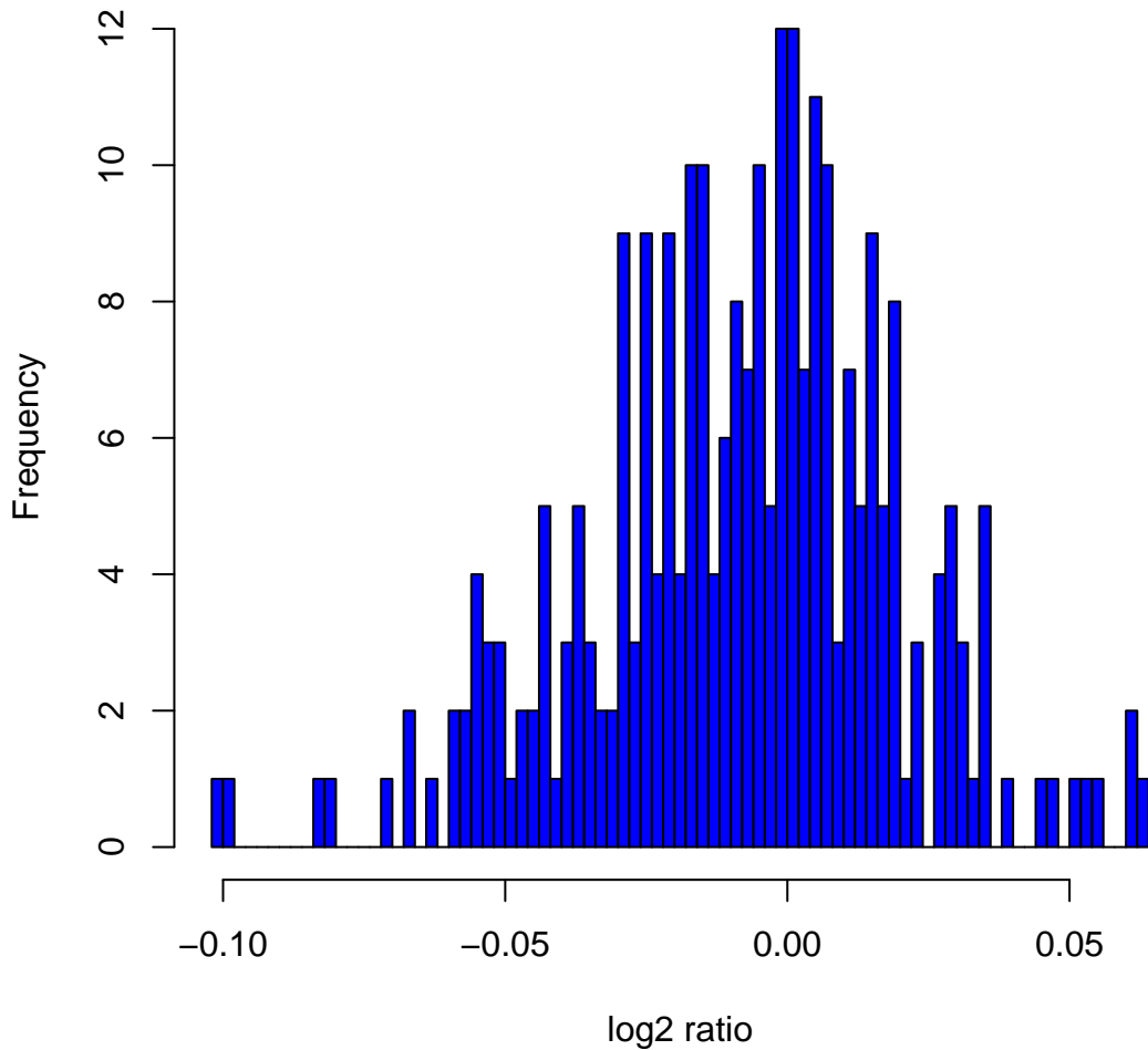
Histogram of \log_2 ratios in 270 HapMap samples at clone Chr6tp-6H6
