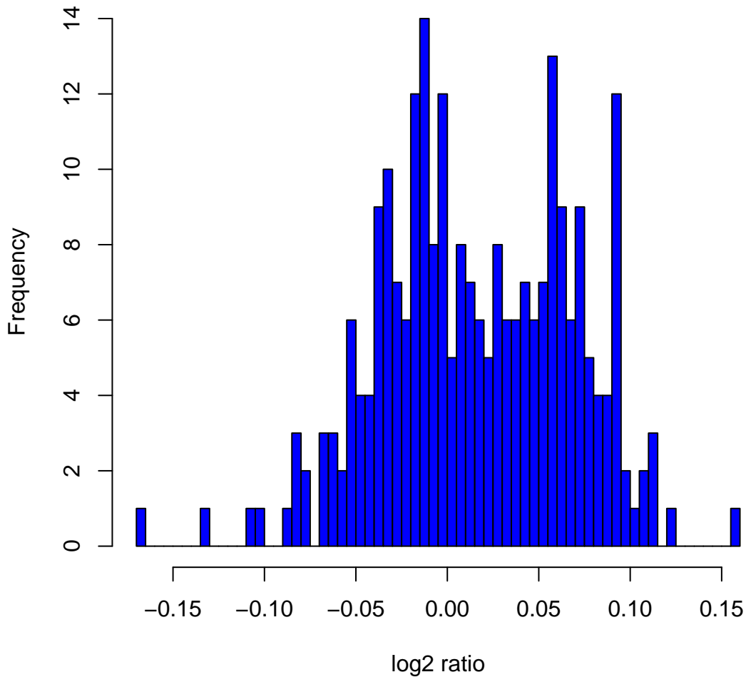
Histogram of log2ratios in 270 HapMap samples at clone Chr6tp-7B2
