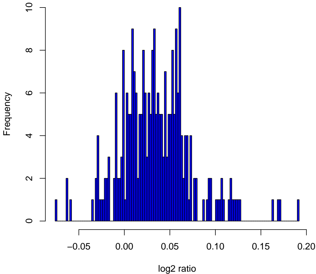
Histogram of log2ratios in 270 HapMap samples at clone Chr6tp-8A1
