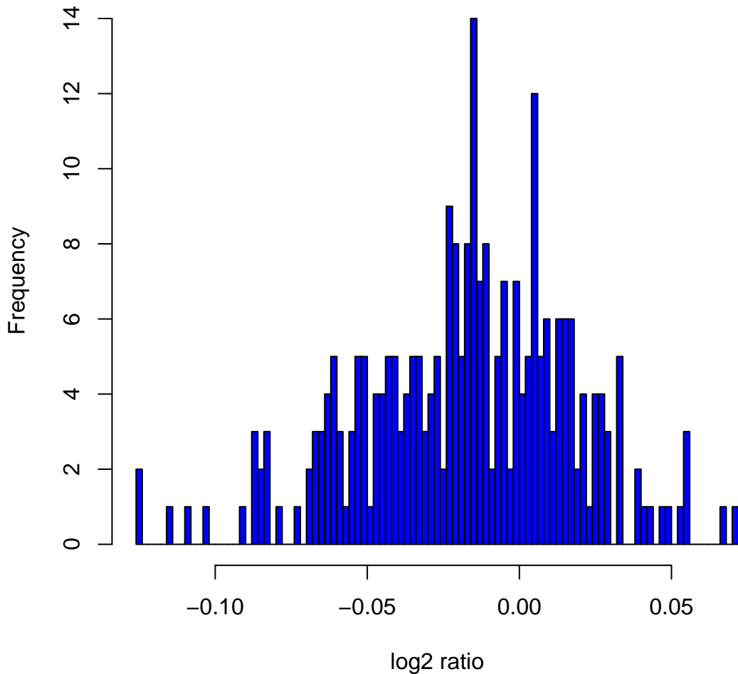
Histogram of log 2 ratios in 270 HapMap samples at clone Chr6tp-8B5
