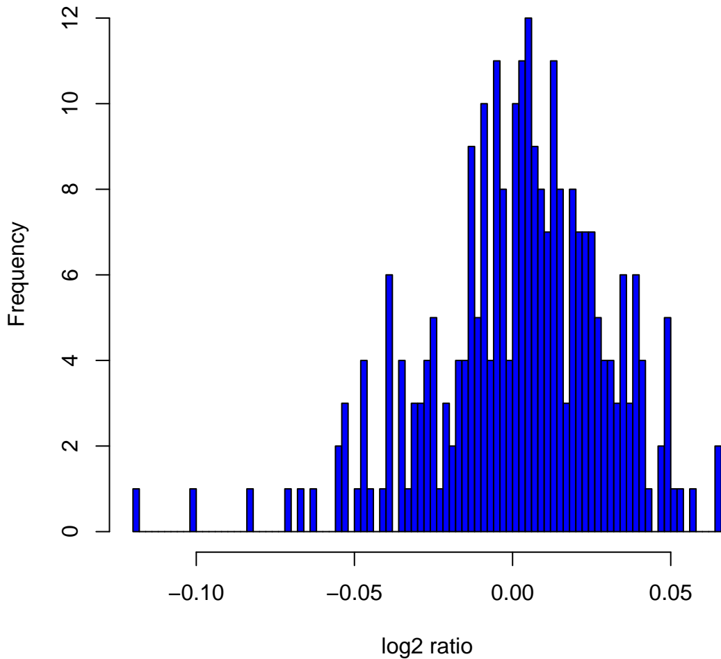
Histogram of log 2 ratios in 270 HapMap samples at clone Chr6tp-8B7
