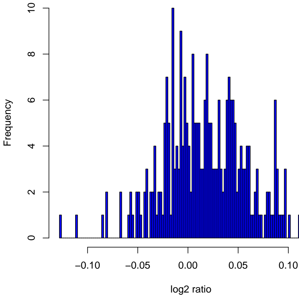
Histogram of log2ratios in 270 HapMap samples at clone Chr6tp-8E6
