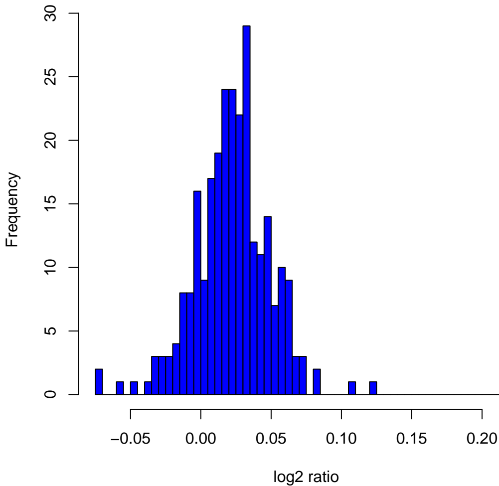
Histogram of log 2 ratios in 270 HapMap samples at clone Chr6tp-8E8
