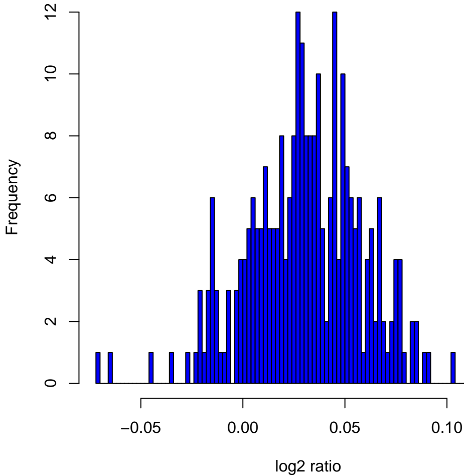
Histogram of log2ratios in 270 HapMap samples at clone Chr6tp-8F2
