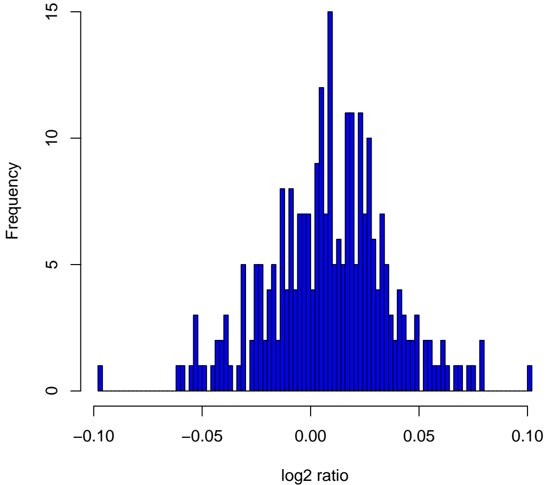
Histogram of log2ratios in 270 HapMap samples at clone Chr6tp-8F6
