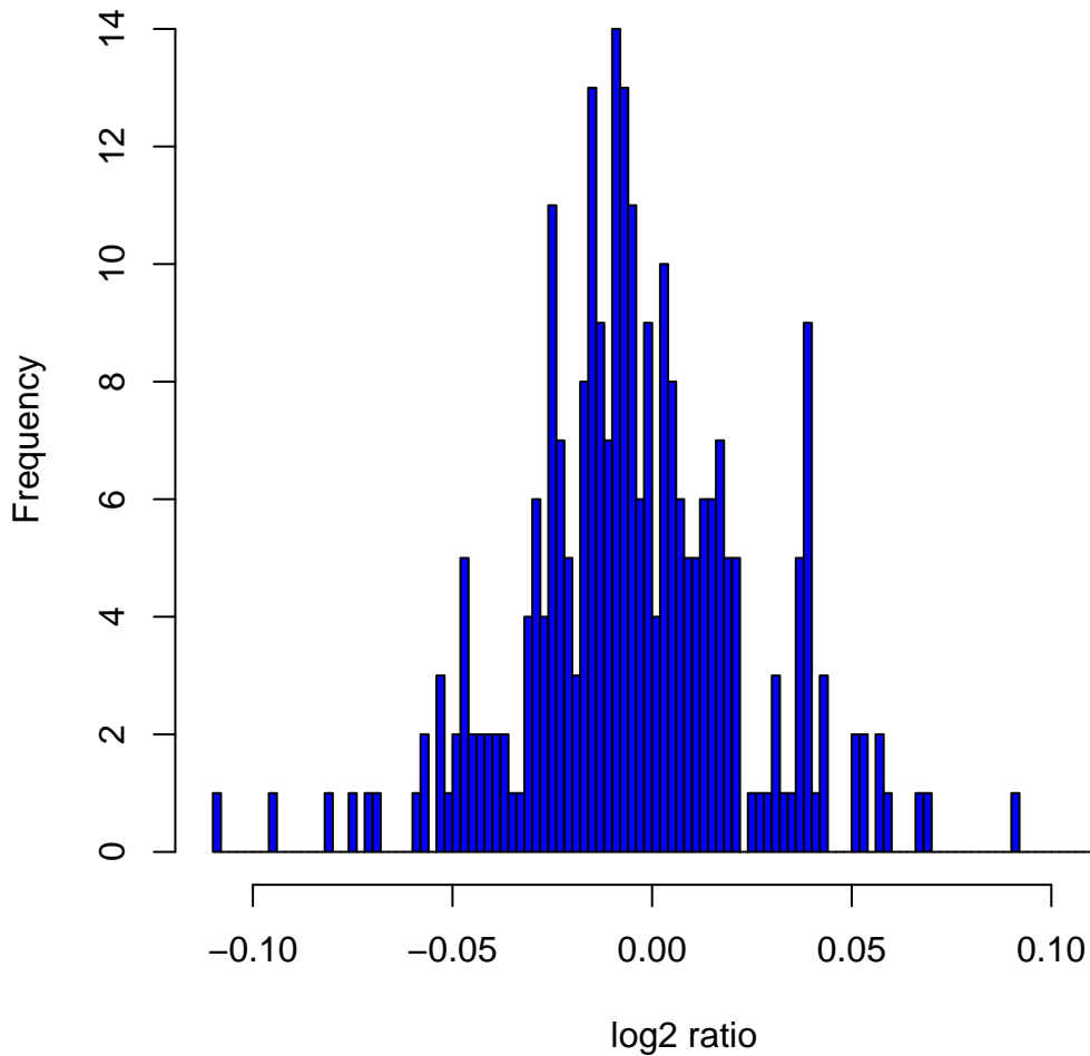
Histogram of log 2 ratios in 270 HapMap samples at clone Chr6tp-8H3
