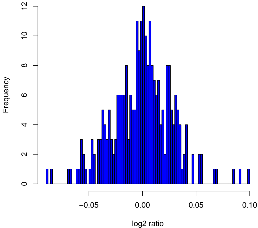
Histogram of log 2 ratios in 270 HapMap samples at clone Chr6tp-8H5
