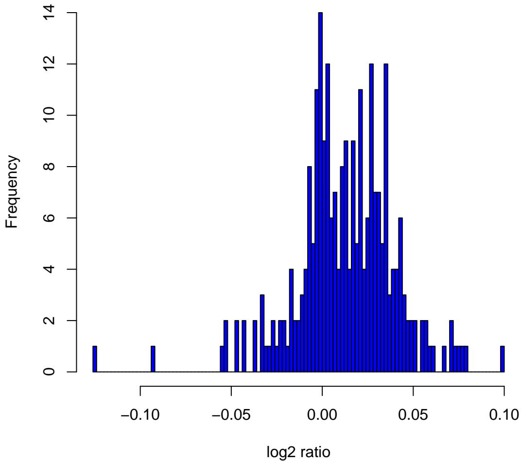
Histogram of log 2 ratios in 270 HapMap samples at clone Chr6tp-9A5
