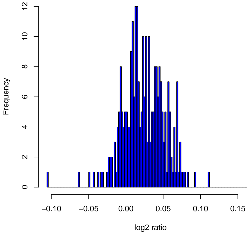
Histogram of log 2 ratios in 270 HapMap samples at clone Chr6tp-9A6
