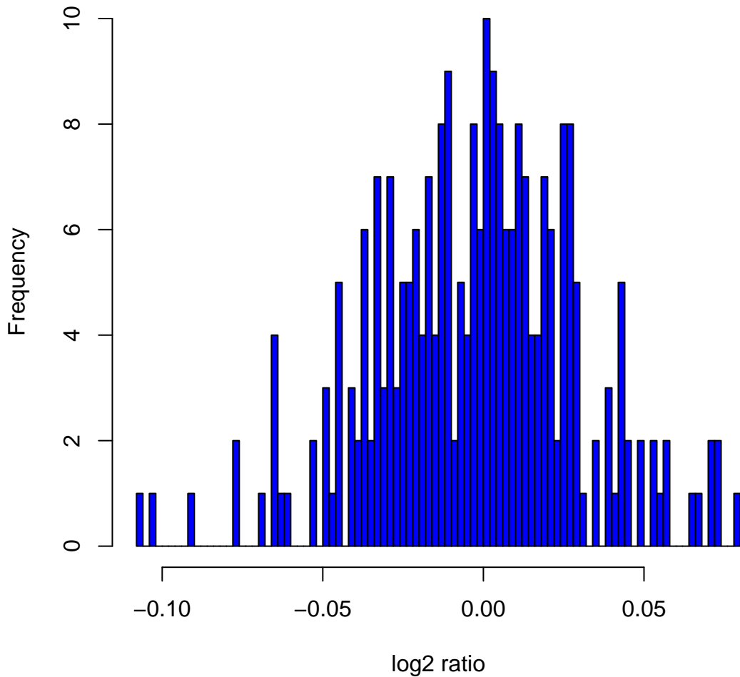
Histogram of log 2 ratios in 270 HapMap samples at clone Chr6tp-9B11
