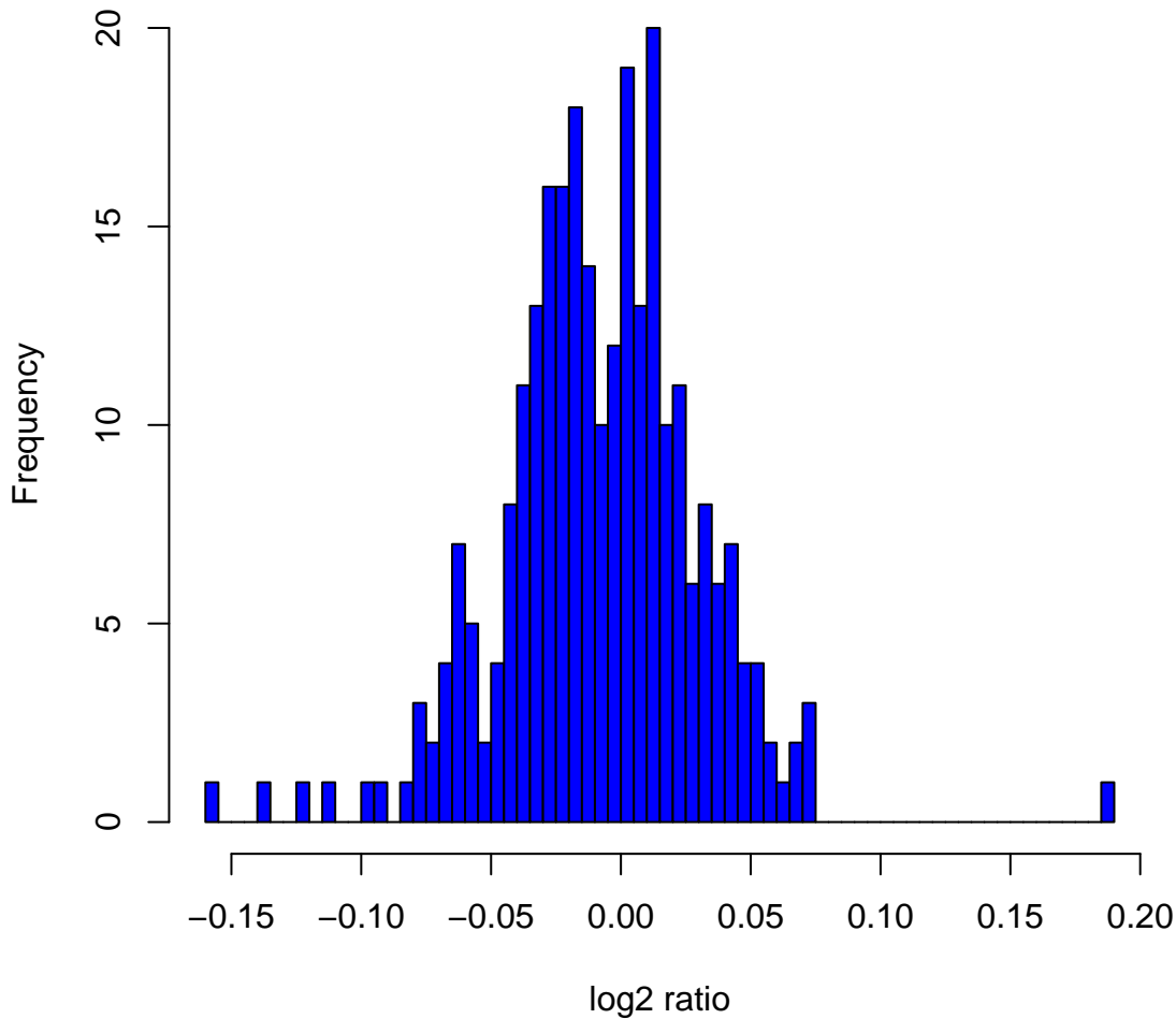
Histogram of log 2 ratios in 270 HapMap samples at clone Chr6tp-9C6
