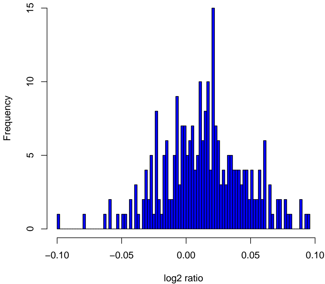
Histogram of log2ratios in 270 HapMap samples at clone Chr6tp-9D12
