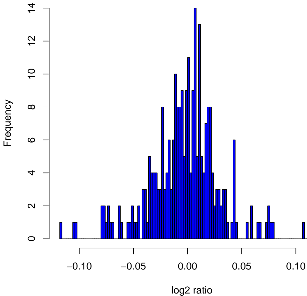
Histogram of log 2 ratios in 270 HapMap samples at clone Chr6tp-9E5
