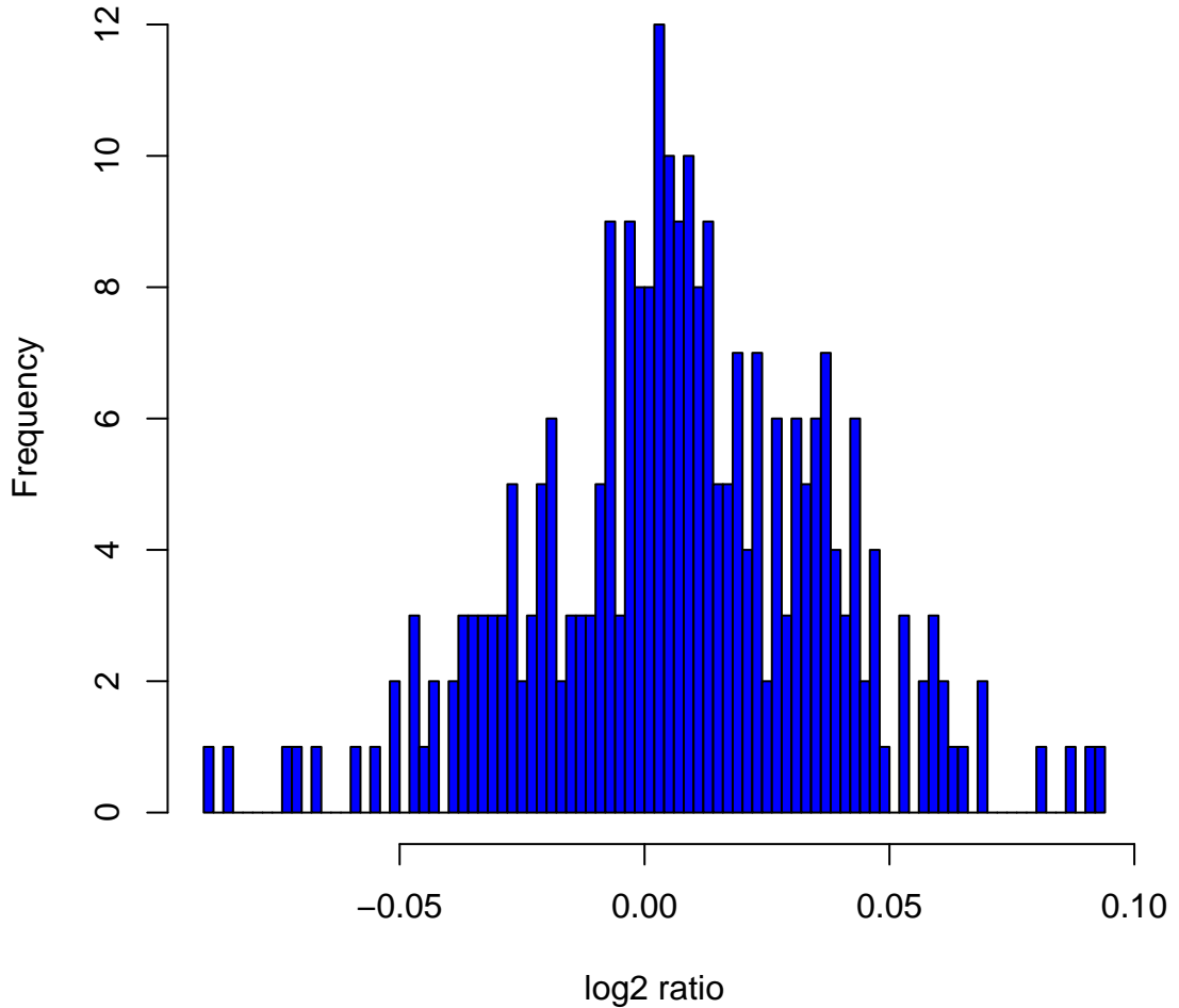
Histogram of log2ratios in 270 HapMap samples at clone Chr6tp-9F6
