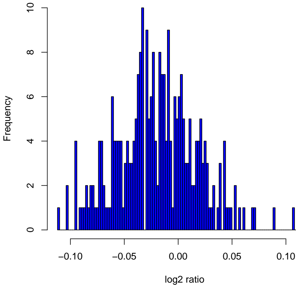
Histogram of log 2 ratios in 270 HapMap samples at clone Chr6tp-9G10
