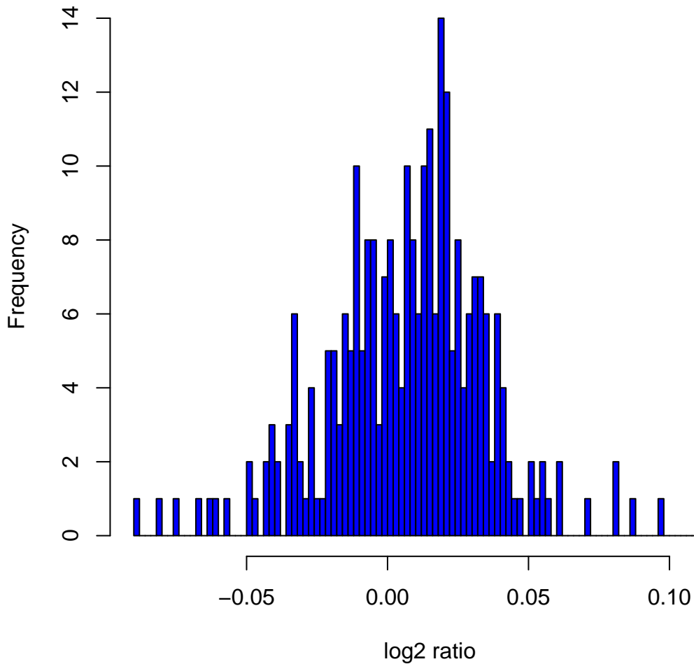
Histogram of log 2 ratios in 270 HapMap samples at clone Chr6tp-9G4
